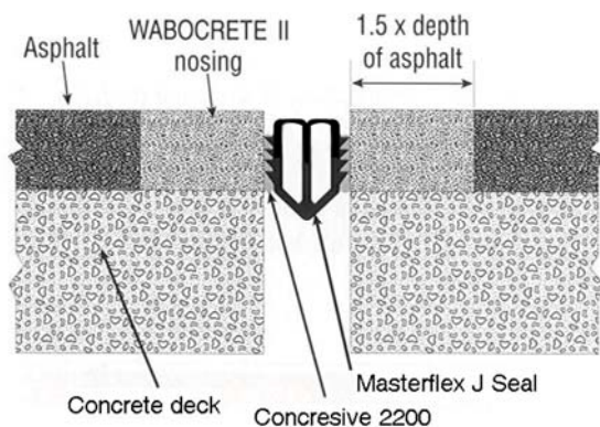
Figure 2 : Section through MASTERFLEX J SEAL
