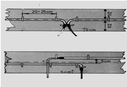
Figure 4: Clamping of hose
