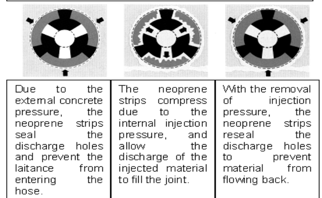
Figure 2: Action of neoprene 'one-way' valves
