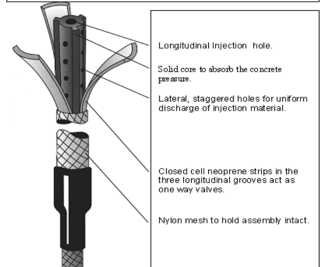
Figure 2: Action of neoprene 'one-way' valves
